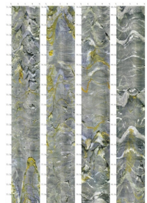
Actual data of 60mm diameter drilling hole
