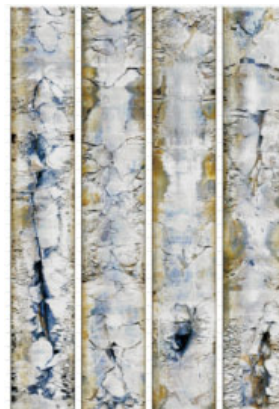
Measured data of 76mm diameter drilling hole
