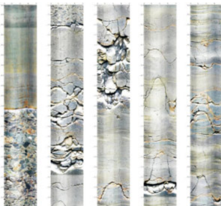
Measured data of 91mm diameter borehole
