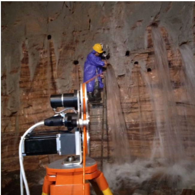
Horizontal hole inspection of tunnel engineering
